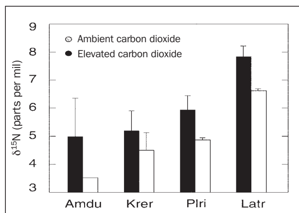
Figure 4. The nitrogen isotope ratio ( \delta^{15}\text{N} ) of leaves of Ambrosia dumosa (Amdu), Krameria erecta (Krer), Pleuraphis rigida (Plri), and Larrea tridentata (Latr) at the Nevada Desert FACE (free-air carbon dioxide enrichment) facility, September 1999. Modified from Billings and colleagues (2002).
