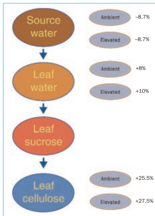
Figure 6. Oxygen isotope ratios of Liriodendron tulipifera and its source water (relative to Vienna standard mean ocean water) grown under elevated (+300 parts per million) and ambient concentrations of carbon dioxide. Data from Cooper and Norby (1994).
