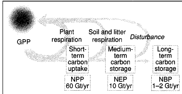
Terrestrial carbon uptake and storage.
