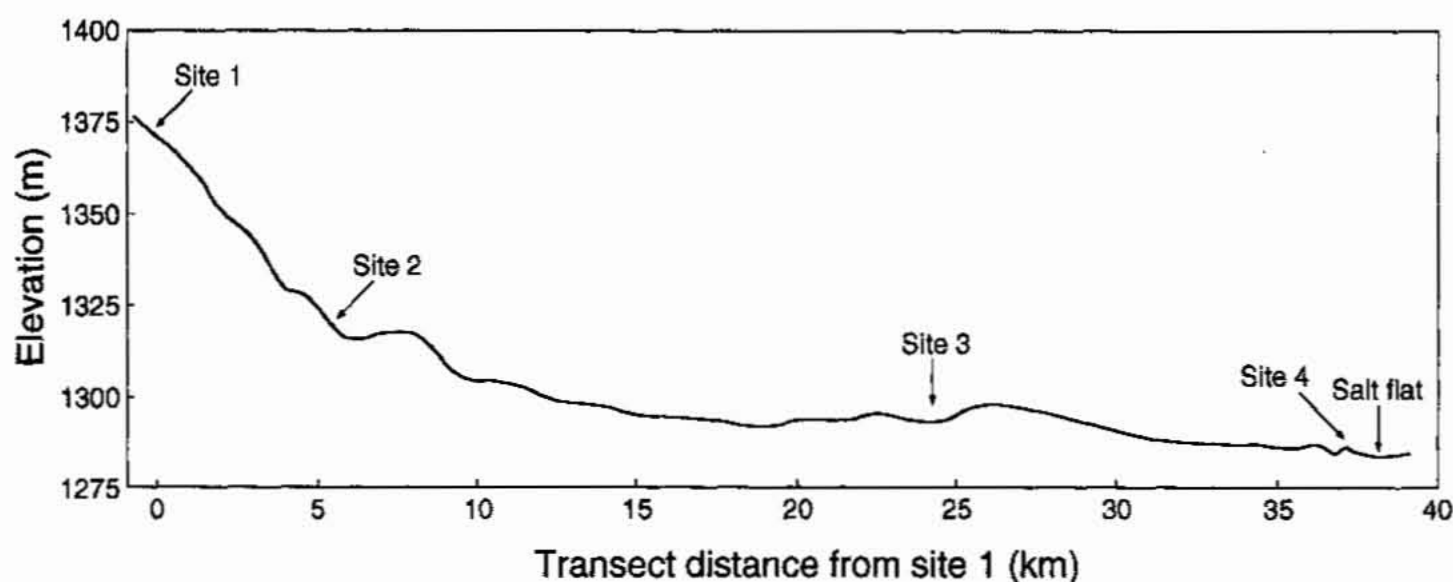
Fig. 1. Study transect in cross section. Shown is the topography over the transect and localities of each study site based on the approximate linear distance from site 1.
