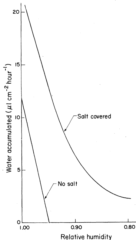
Fig. 2 (left). Scanning electron micrograph of leaf surface of Nolana mollis , showing salt gland in a depression. Fig. 3 (right). Simulations of hourly water uptake by leaves of Nolana at different relative humidities. The environmental conditions used for the energy budget simulations were typical of nighttime conditions. Leaf resistance, 99 \text{ sec cm}^{-1} ; wind speed, 50 \text{ cm sec}^{-1} ; downward infrared radiation, 279 \text{ W m}^{-2} ; and air and soil temperatures, 15^{\circ}\text{C} . The water uptake under natural or "no salt" conditions is the result of dew formation. The salt concentration of the leaf was set as saturated sodium chloride (osmotic potential about -40 \text{ MPa} ). Simulations were done on a minute-by-minute basis and totaled for an hour.
