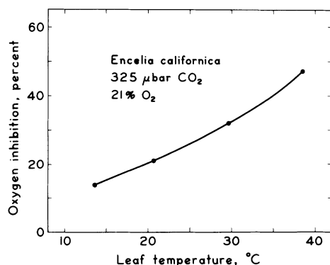
FIG. 4. Oxygen inhibition of E. californica in 21% O 2 as a function of leaf temperature. The CO 2 pressure was held constant at 325 μbars.
