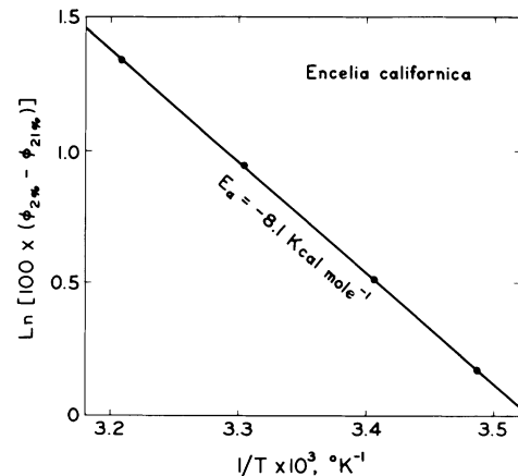
FIG. 5. Arrhenius plot of the difference in quantum yield as determined in 2 and 21% O 2 and at 325 μbar CO 2 for E. californica (C 3 ).
