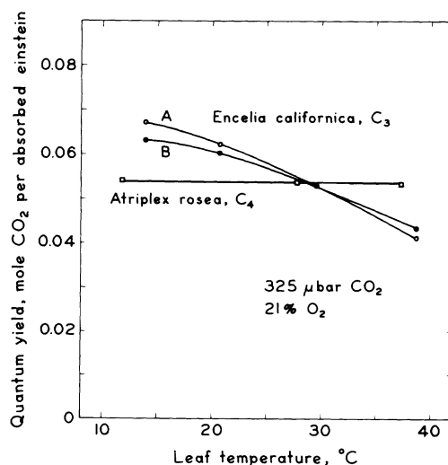
FIG. 3. Quantum yield for CO 2 uptake in E. californica (C 3 ) and A. rosea (C 4 ) as a function of leaf temperature. Curve A of E. californica represents the measured quantum yields and curve B represents the quantum yields adjusted for changes in liquid phase solubilities of CO 2 and O 2 . The CO 2 pressure was held constant at 325 μbar and O 2 concentration was 21%.
