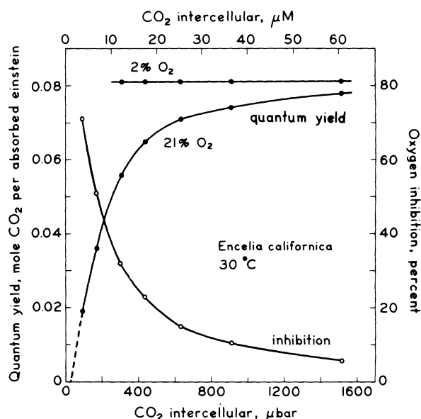
FIG. 2. Quantum yield for CO 2 uptake in E. californica (C 3 ) determined as a function of intercellular CO 2 pressure in 21 and 2% O 2 (●) and O 2 inhibition of quantum yield in 21% O 2 as a function of intercellular CO 2 pressure (○). Leaf temperature was 30 C.
