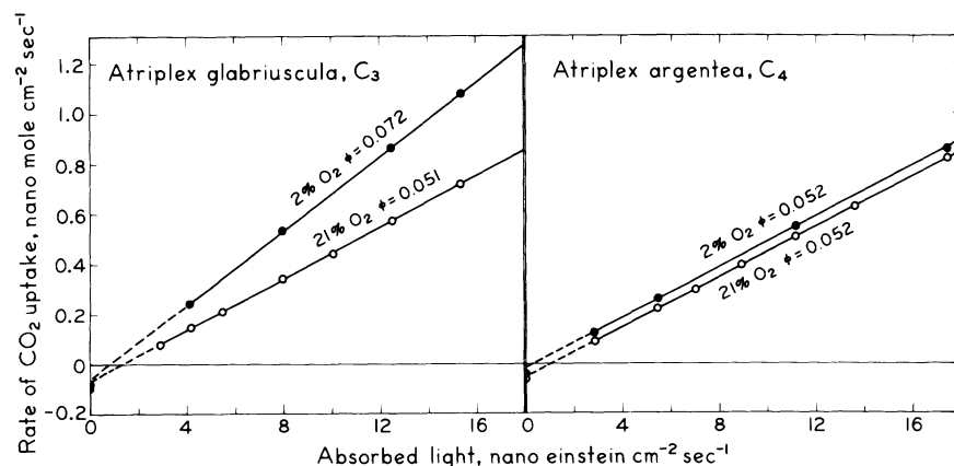
FIG. 1. Rate of CO 2 uptake in A. glabriuscula (C 3 ) and A. argentea (C 4 ) versus absorbed quantum flux in 21 and 2% O 2 . Leaf temperature was 30 C and CO 2 pressure was 325 μbar.
